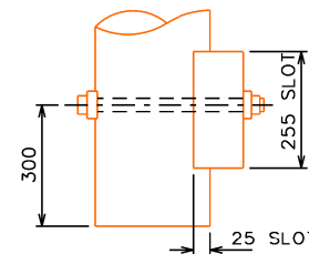
PILOT HOLE 8 DIA x 100 DEEP
