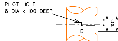
PILOT HOLE 8 DIA x 100 DEEP
