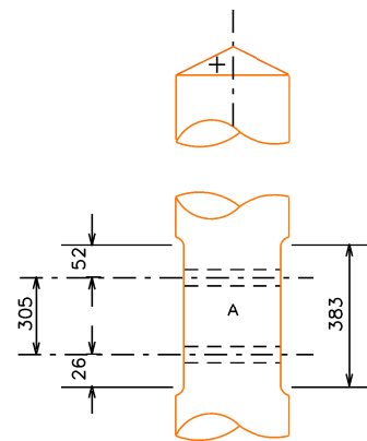
POLE SLOTS ON BOTH SIDES CUT TO GIVE A 100mm FACE
